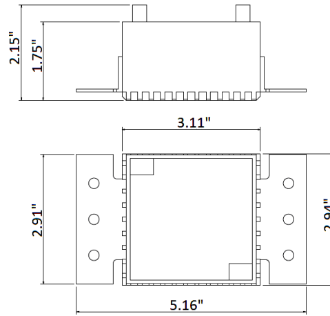
Square Trim Dimension
